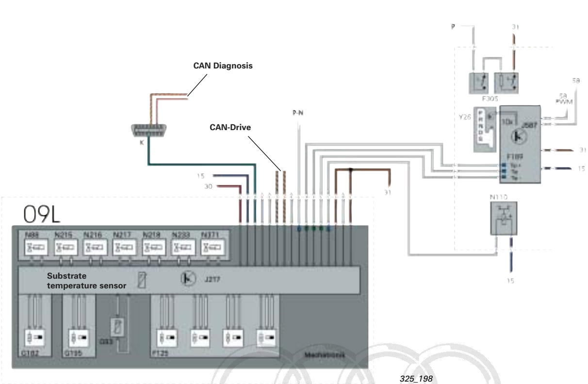
Function diagram for 09L gearbox
