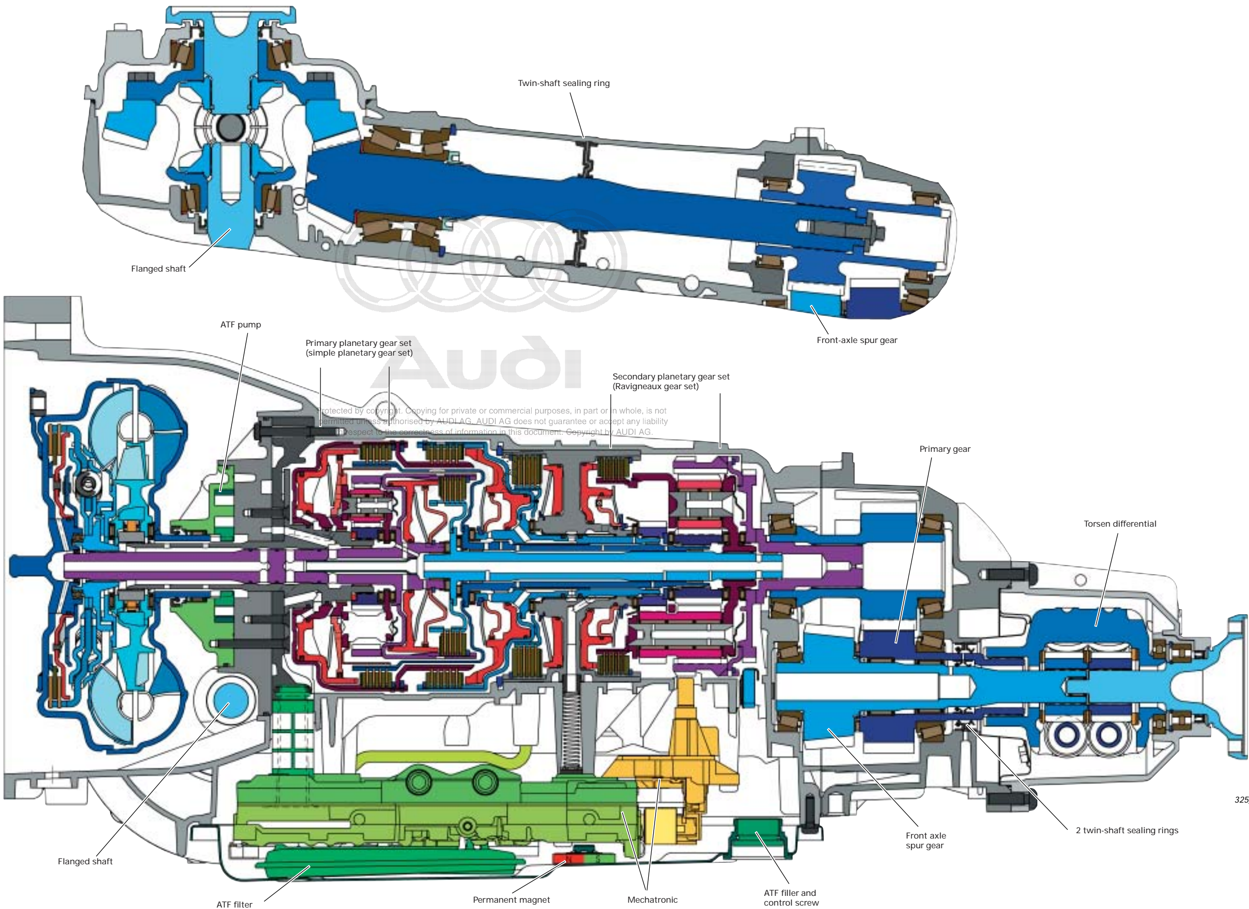
6-gear automatic gearbox 09L
