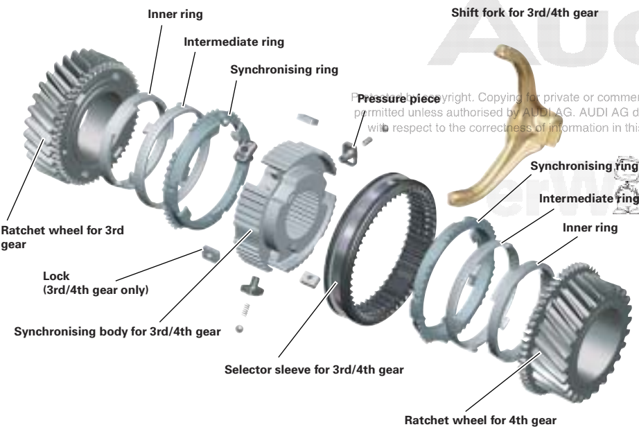
Twin-cone synchronisation 3rd/4th/5th/6th and reverse gear
