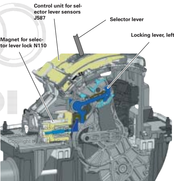
Sectional view from left
