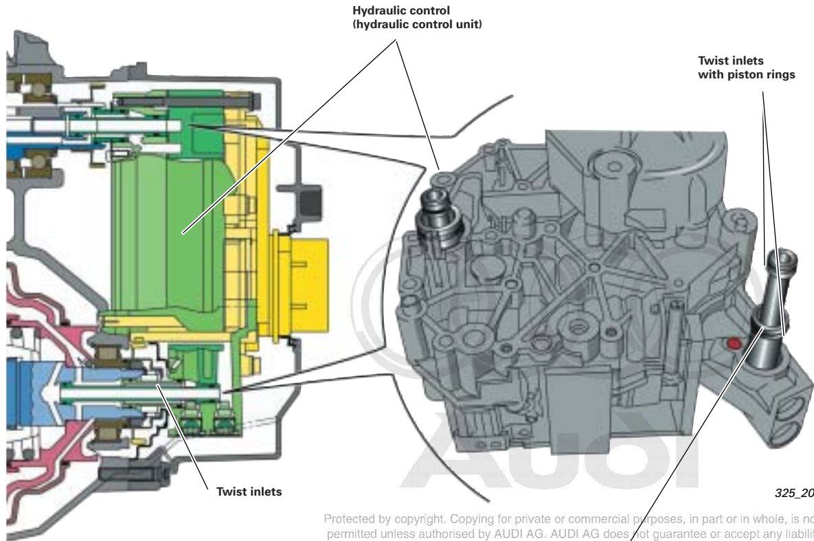
Piston rings in the disc set twist inlets
