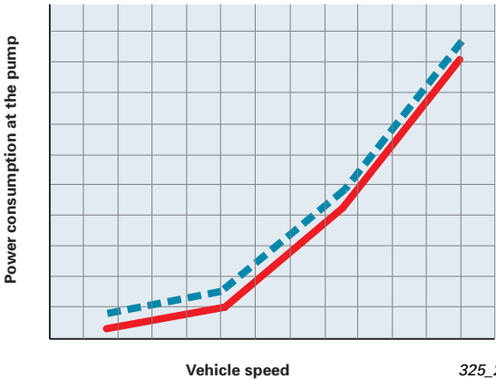
Comparison between crescent-type pump (predecessor) and vane-type pump
