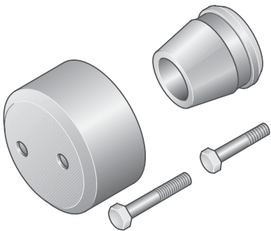
T40048 Assembly device for crankshaft sealing ring
