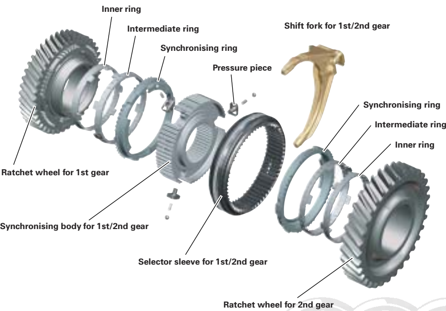
Triple-cone synchronisation 1st/2nd gear
