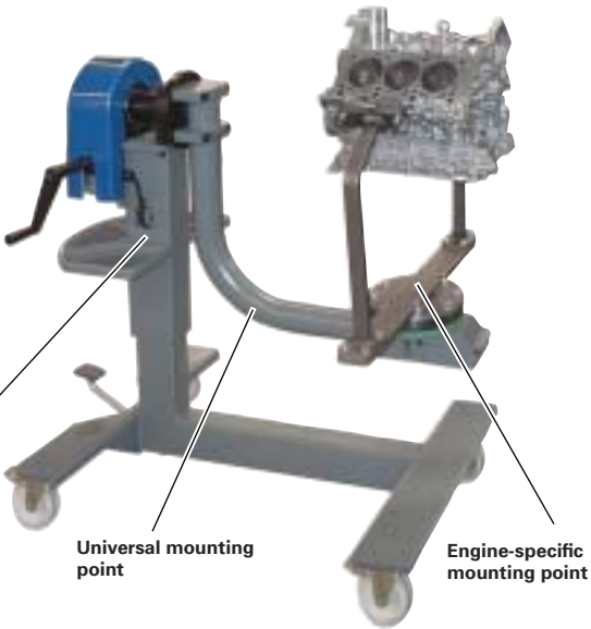
Engine and gearbox holder VAS 6095
