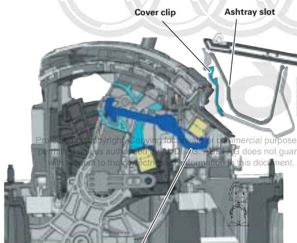
Emergency release lever
