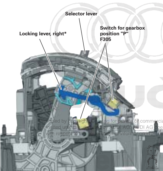
Sectional view from right
