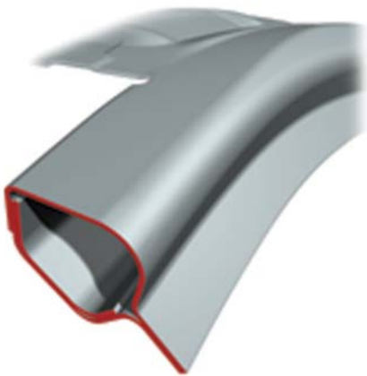
A-post, Audi TT Sheet-aluminium sections (interior/exterior)
