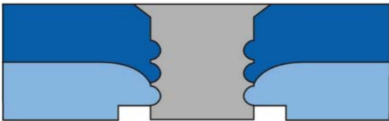
Riveted joint
