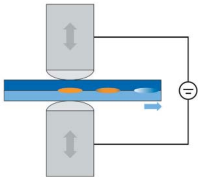
Resistance spot welding process
