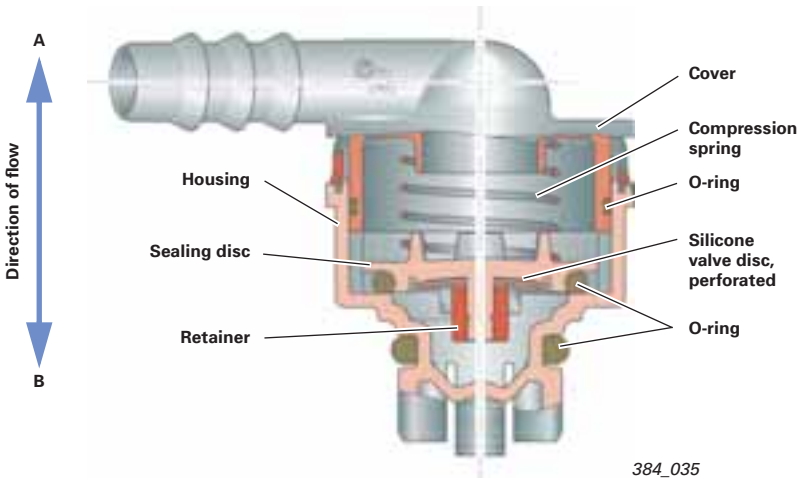
Cutaway view of crankcase breather valve
