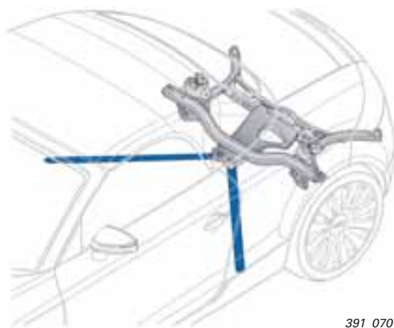
Attachment of the diagonal struts for front-wheel drive
