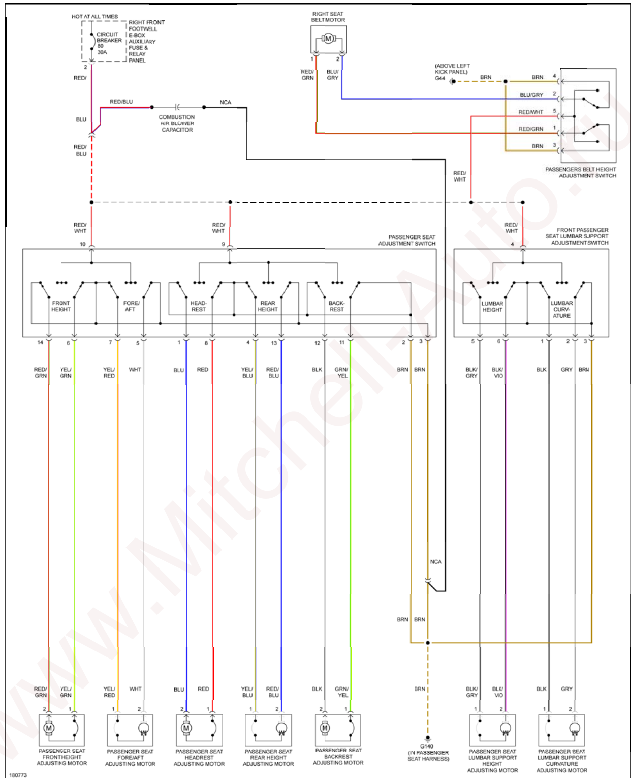
Fig. 49: Passenger Seat Circuit
