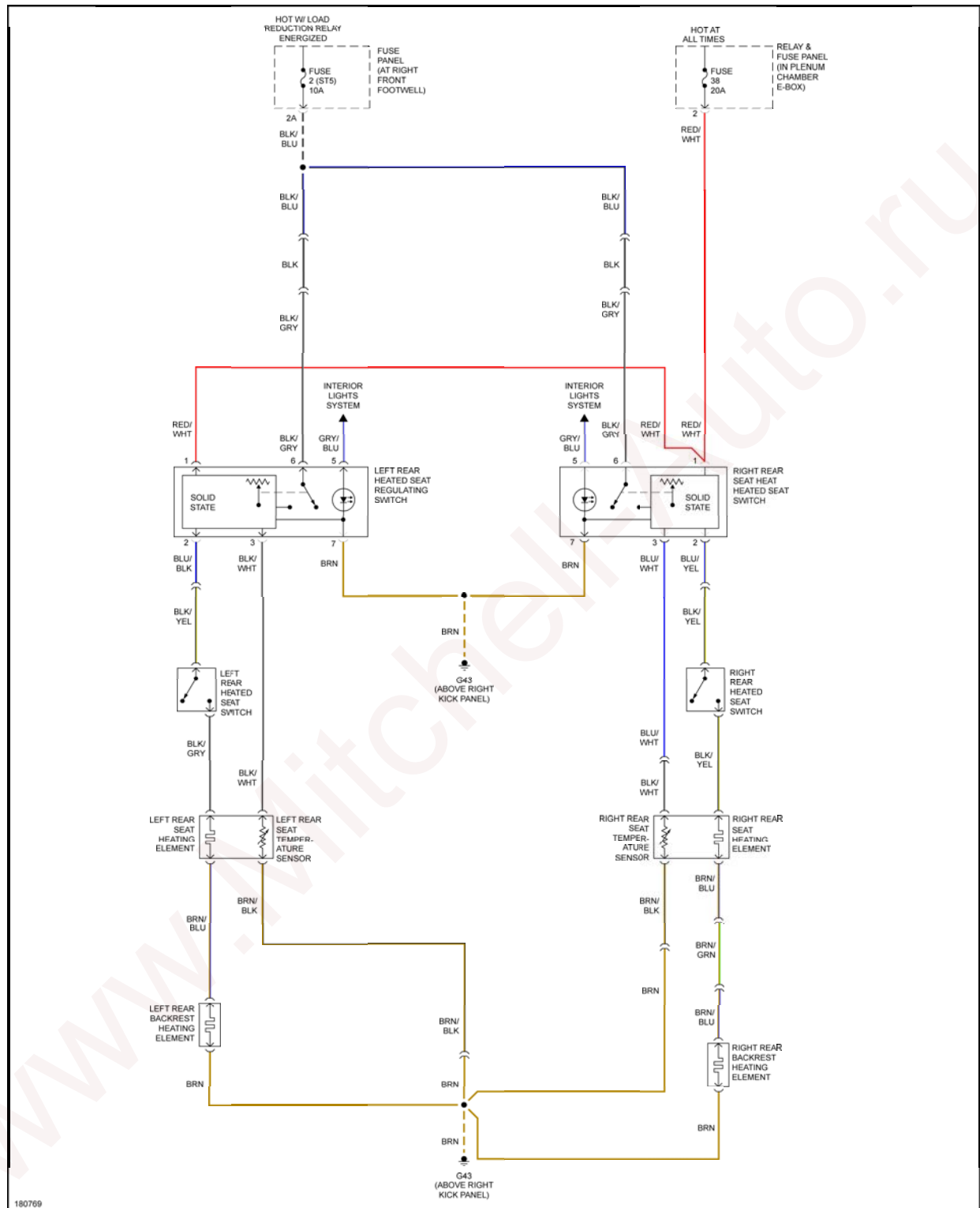
Fig. 50: Rear Heated Seats Circuit
