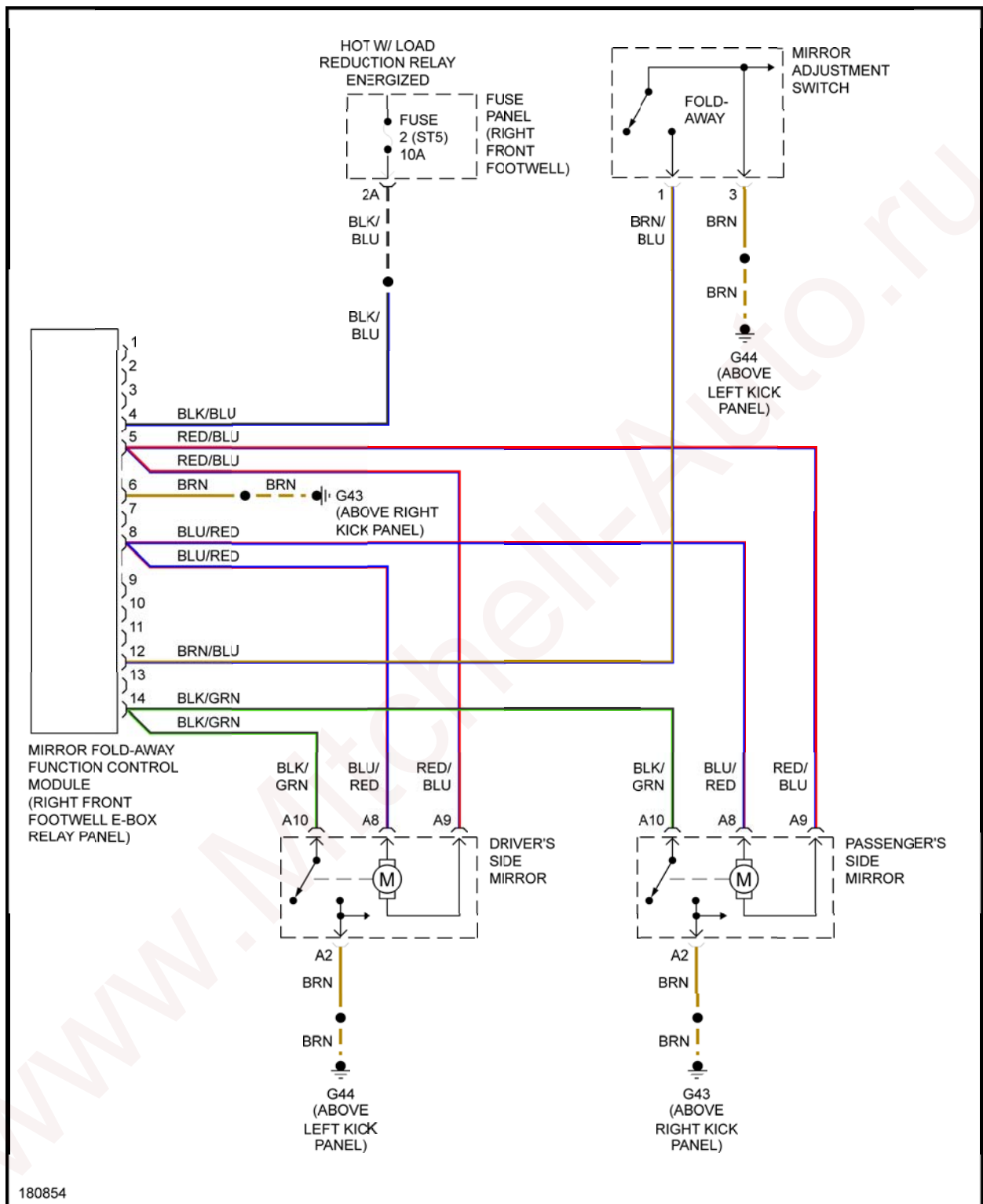
Fig. 45: Fold-back Mirrors Circuit
