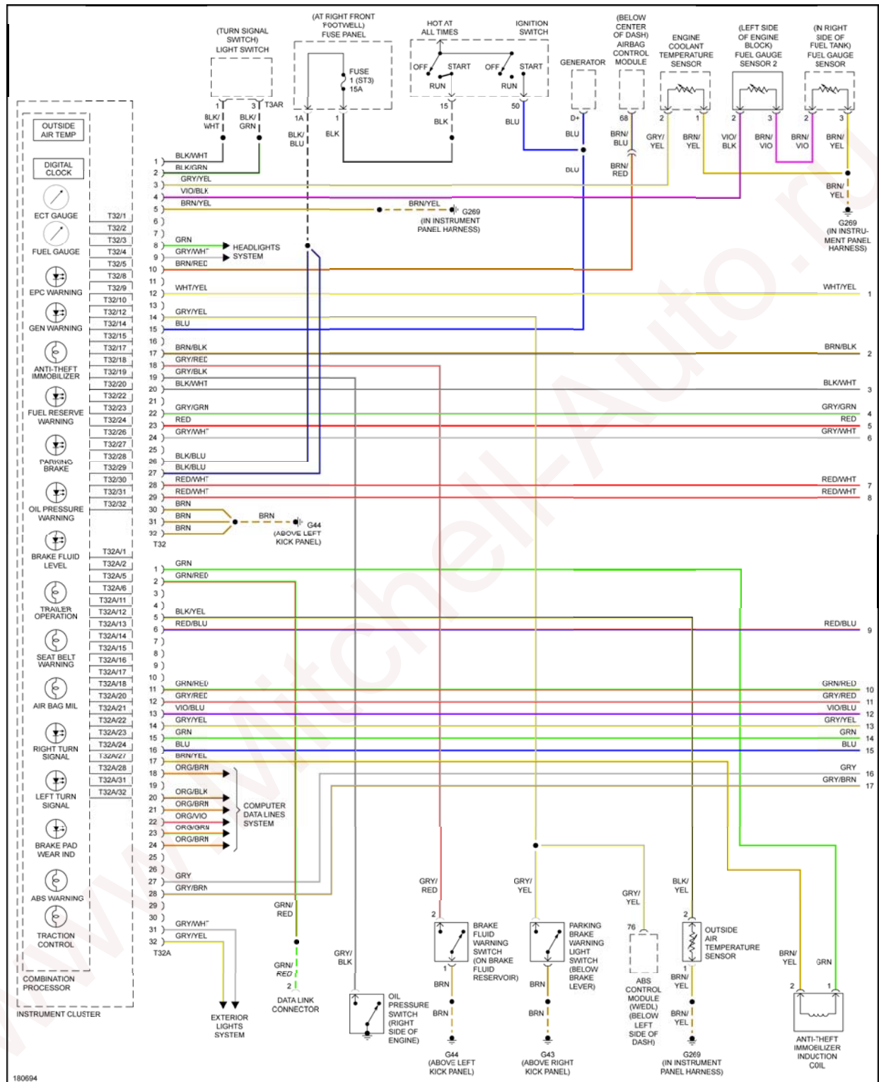
Fig. 27: Instrument Cluster Circuit (1 of 3)
