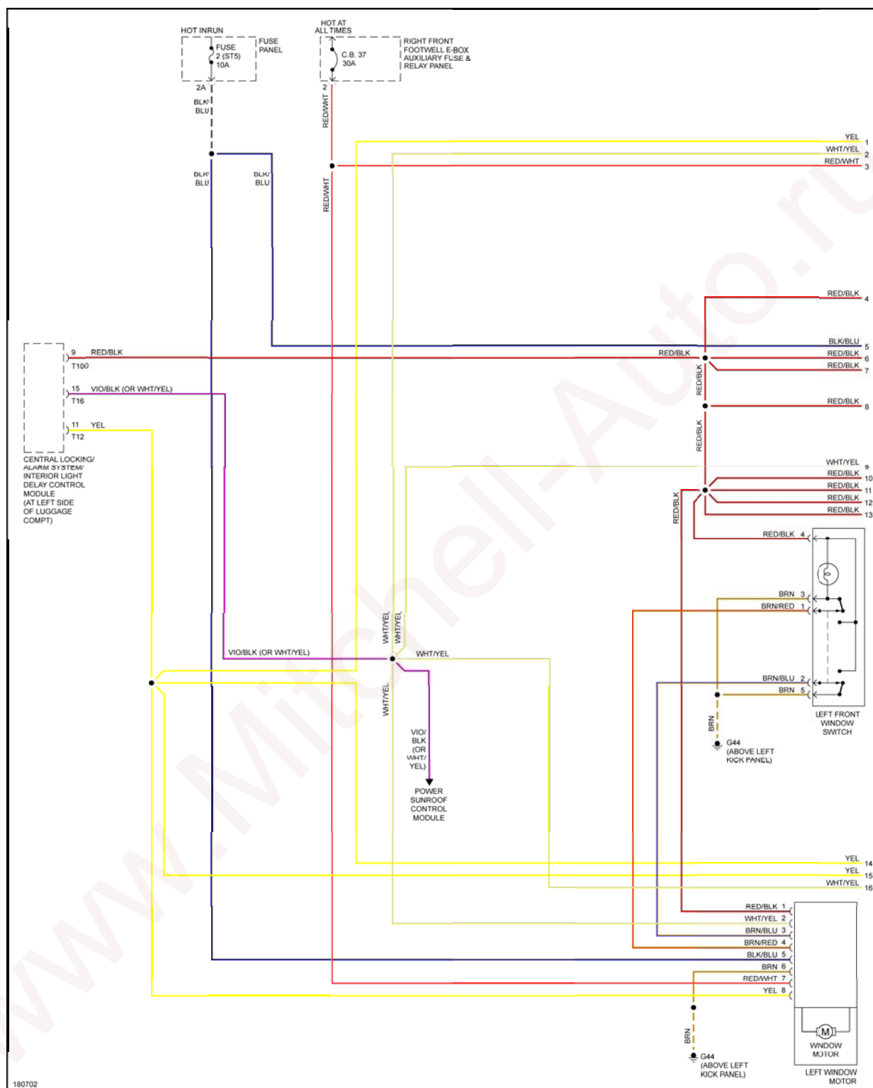
Fig. 54: Power Windows Circuit (1 of 2)
