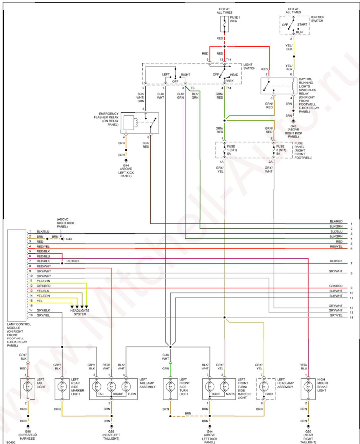
Fig. 17: Exterior Lamps Circuit, W/ DRL (1 of 2)
