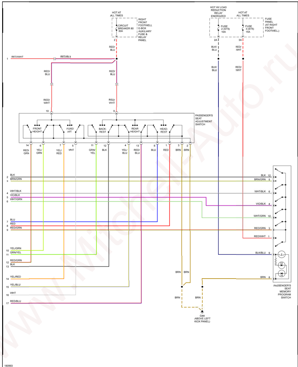
Fig. 38: Passenger's Memory Seat Circuit (2 of 2)
