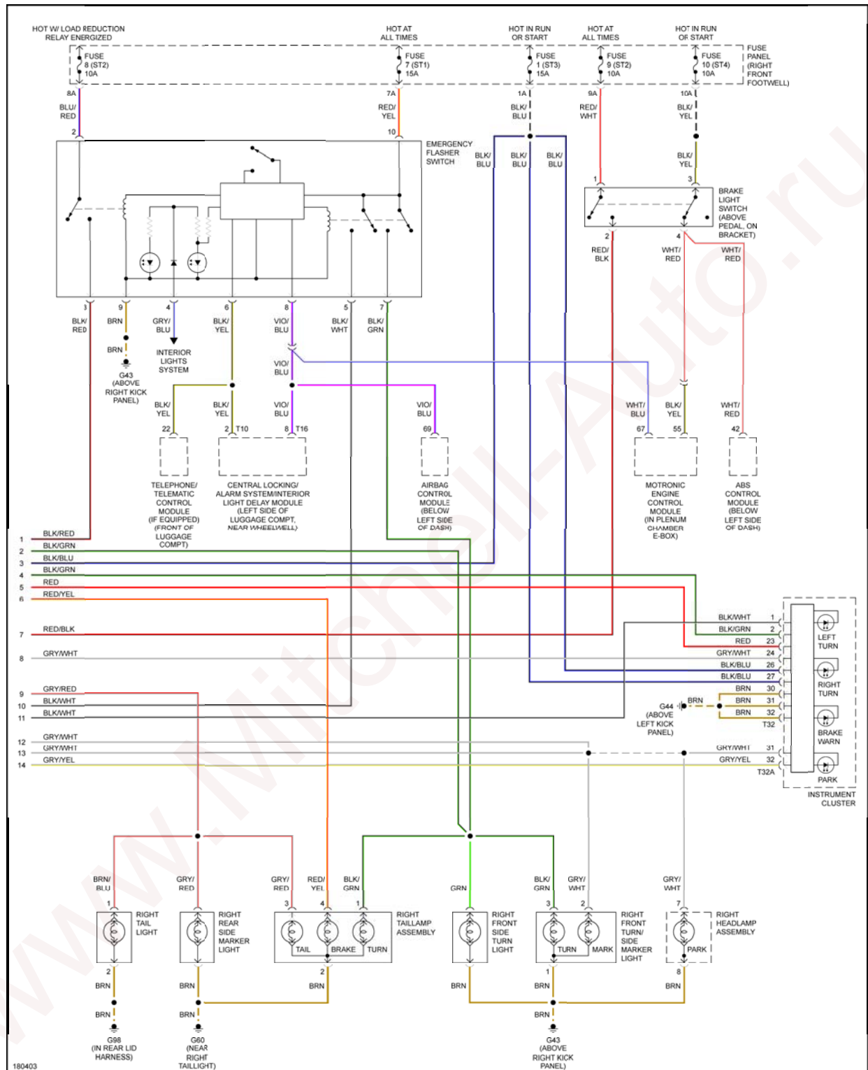
Fig. 20: Exterior Lamps Circuit, W/O DRL (2 of 2)
