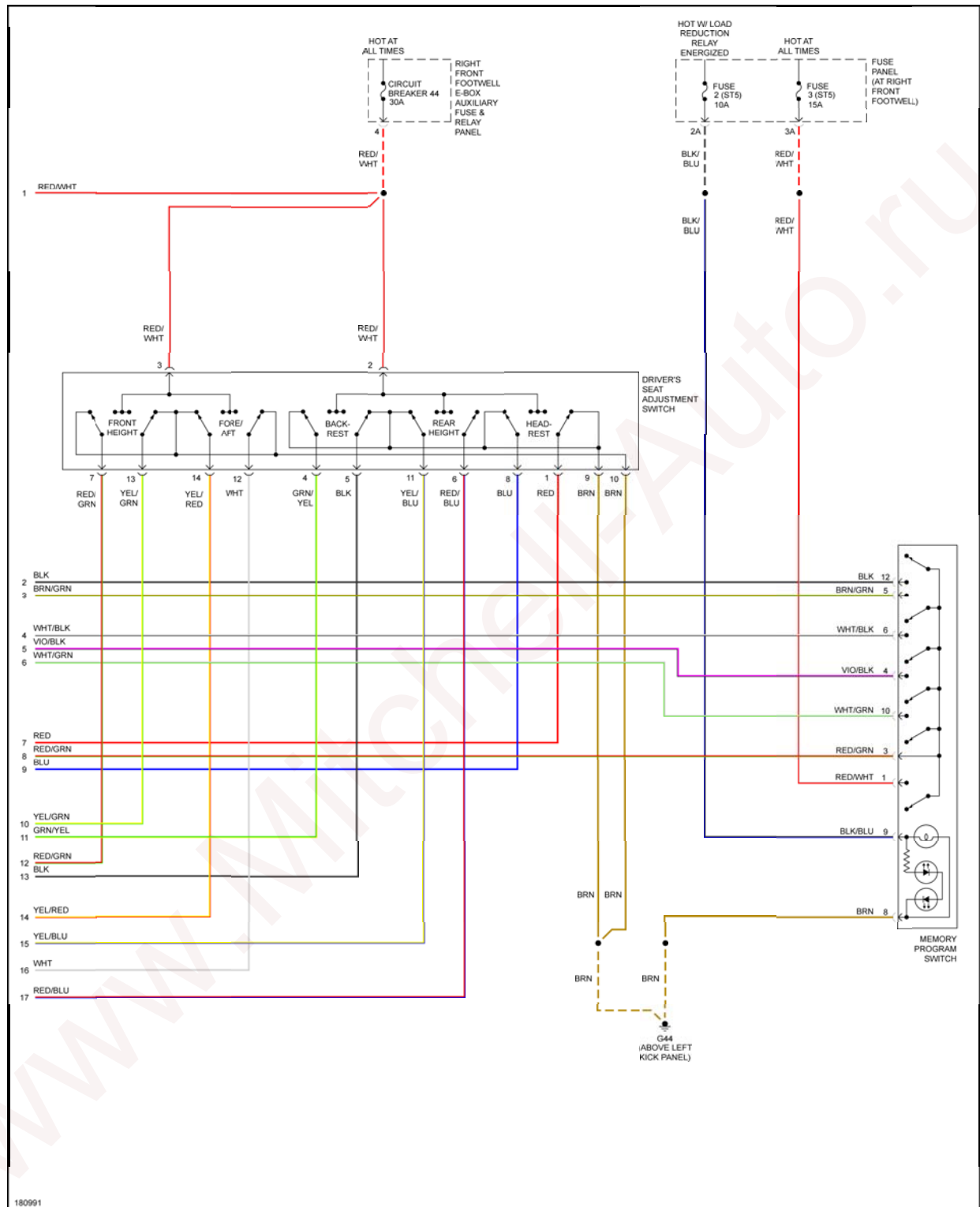
Fig. 34: Driver's Memory Seat Circuit (2 of 2)
