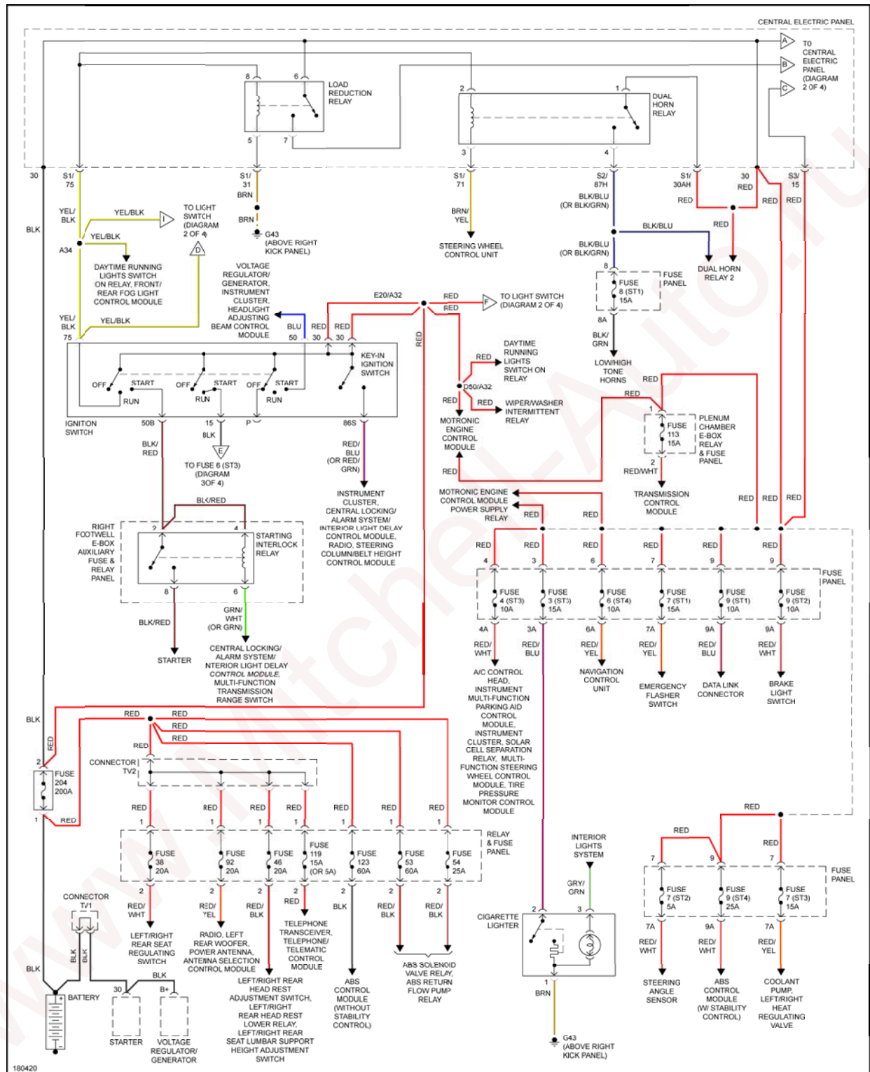
Fig. 40: Power Distribution Circuit (1 of 4)
