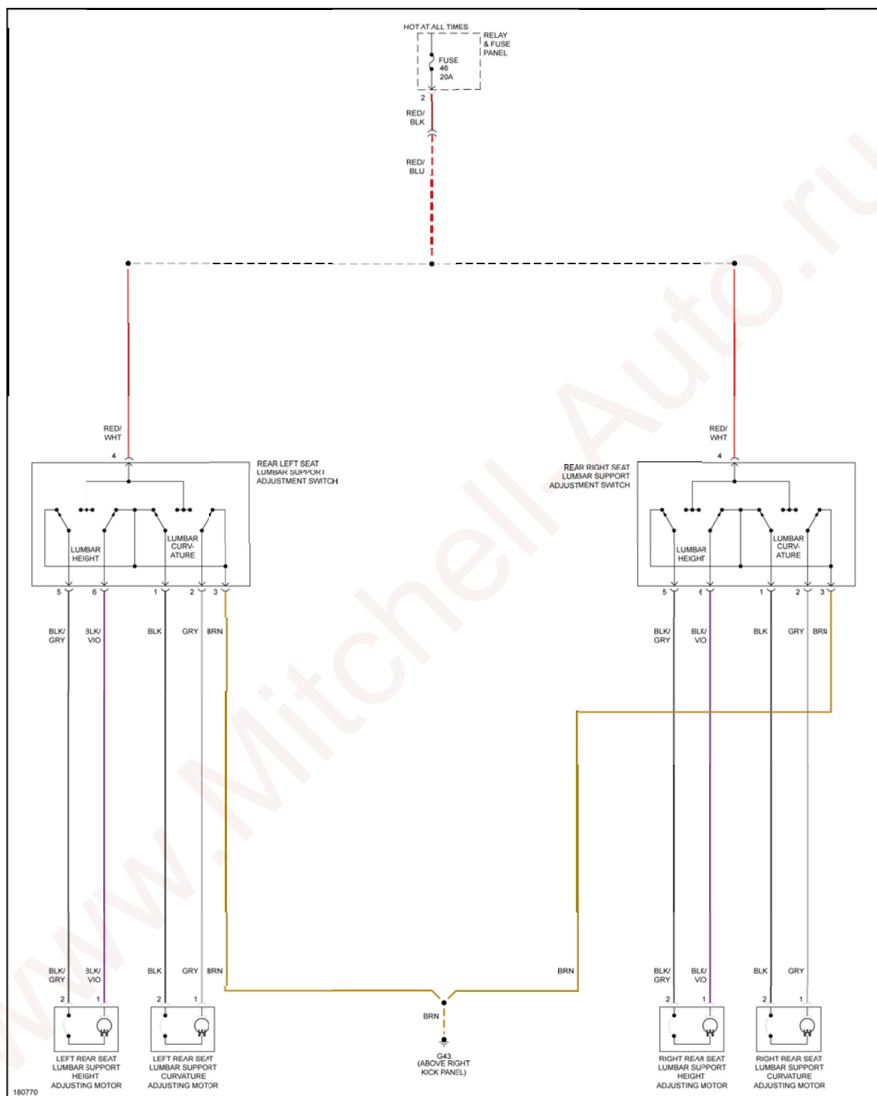
Fig. 51: Rear Lumbar Circuit
