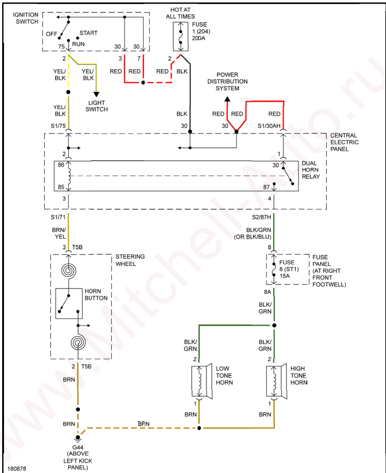
Fig. 26: Horn Circuit, W/O Telematics
