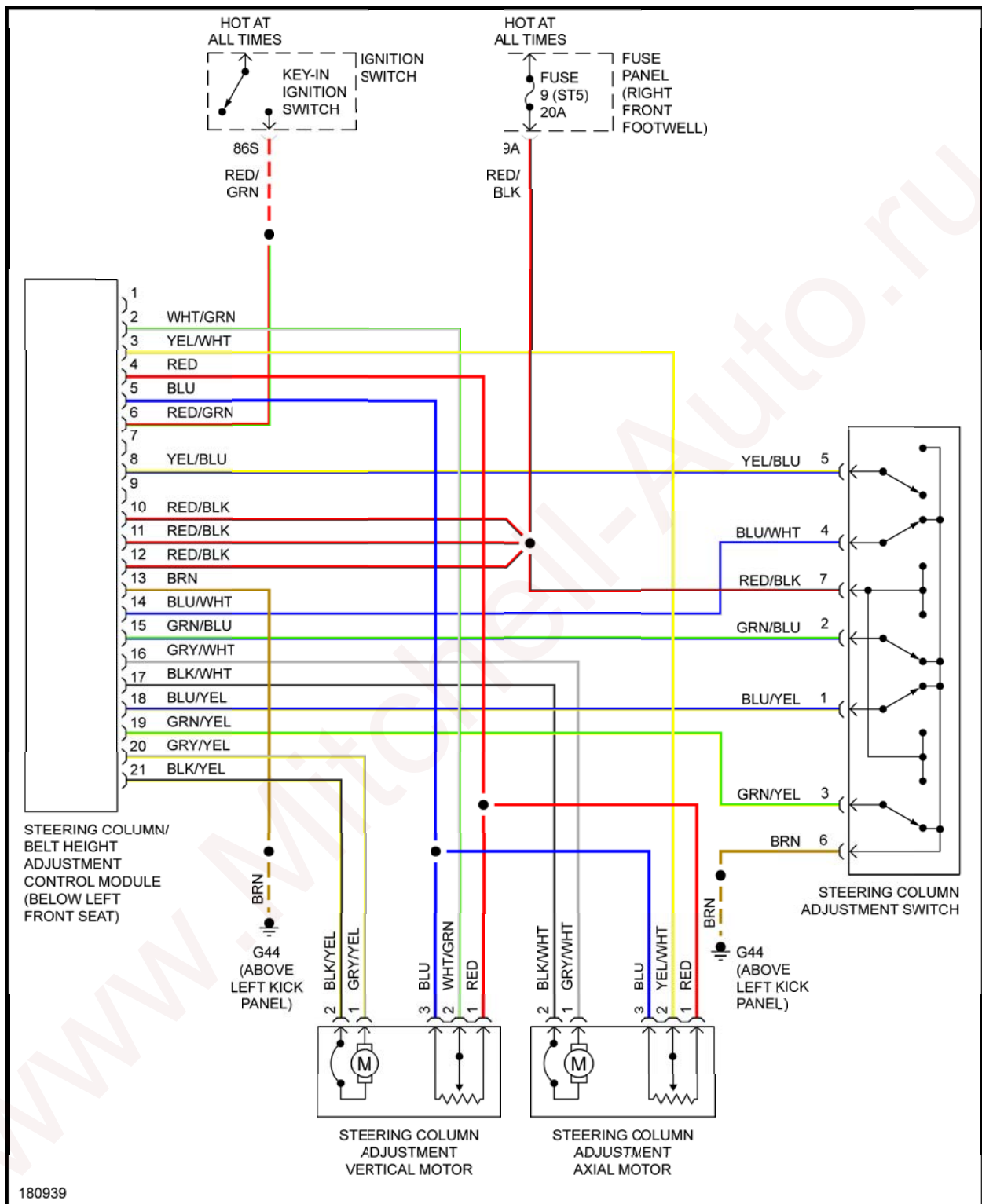
Fig. 11: Power Steering Column Circuit
