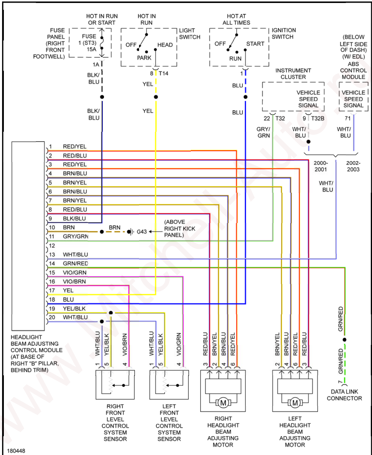
Fig. 23: Headlamp Beam Adjustment Circuit
