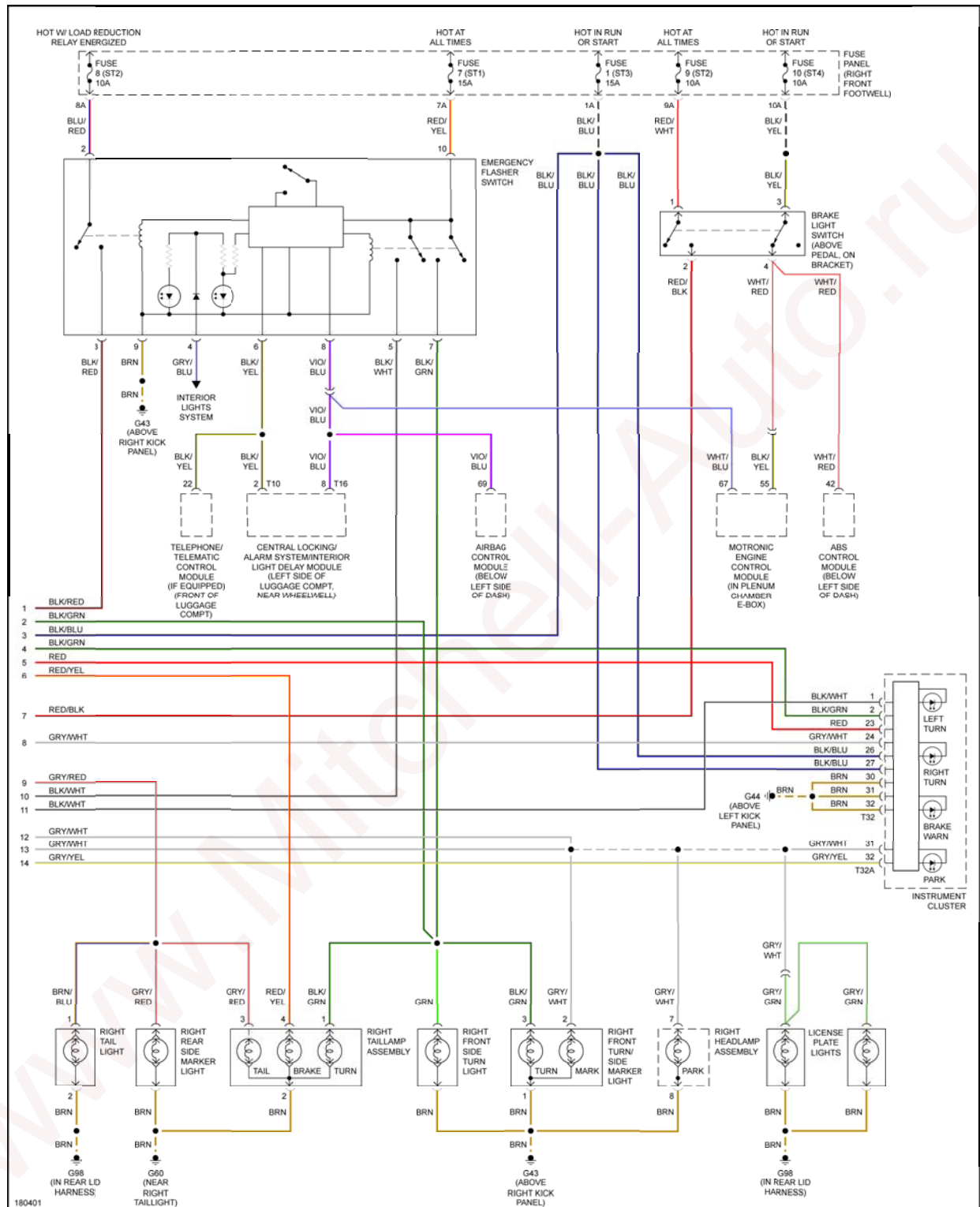
Fig. 18: Exterior Lamps Circuit, W/ DRL (2 of 2)
