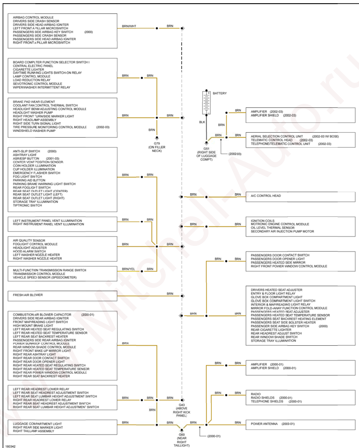
Fig. 21: Ground Distribution Circuit (1 of 2)
