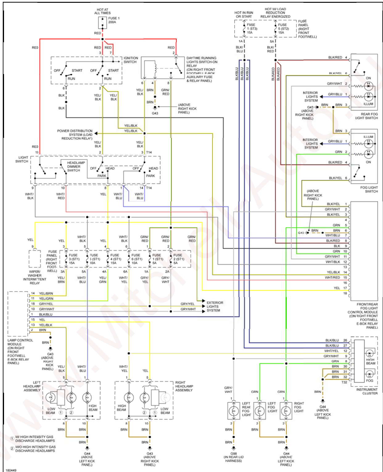
Fig. 24: Headlamps &amp; Fog Lamps Circuit, W/ DRL
