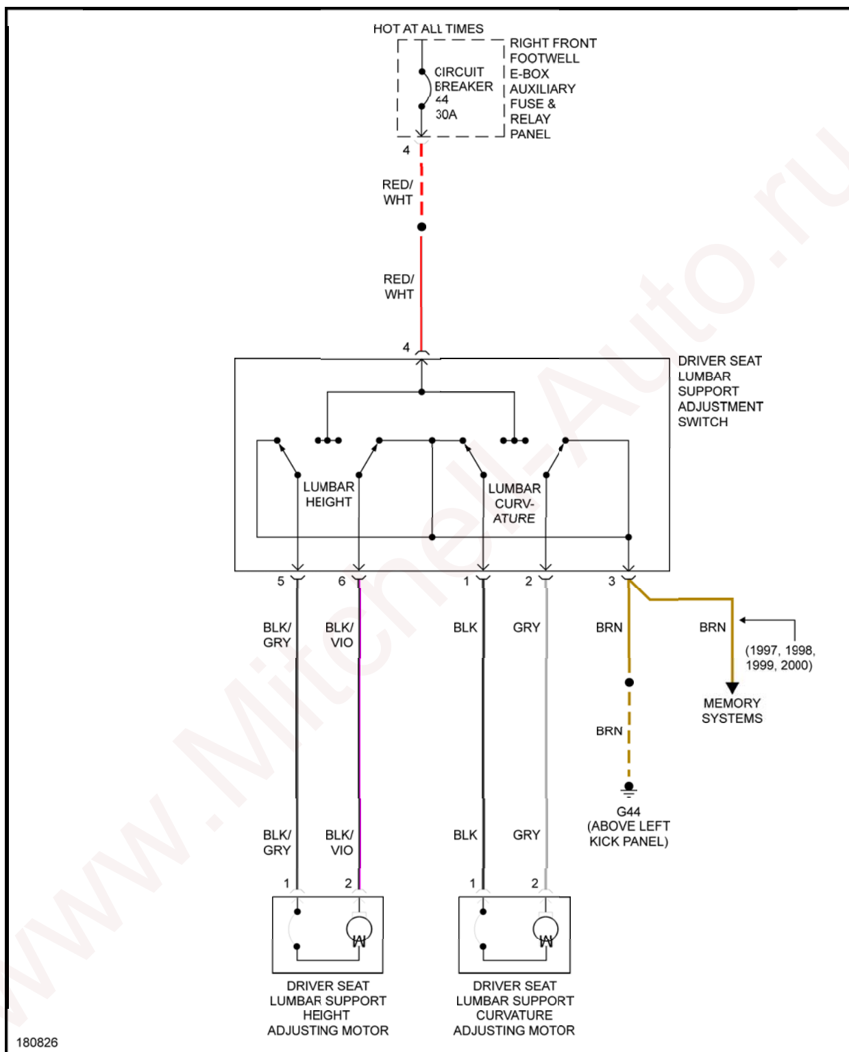
Fig. 46: Driver's Lumbar Circuit
