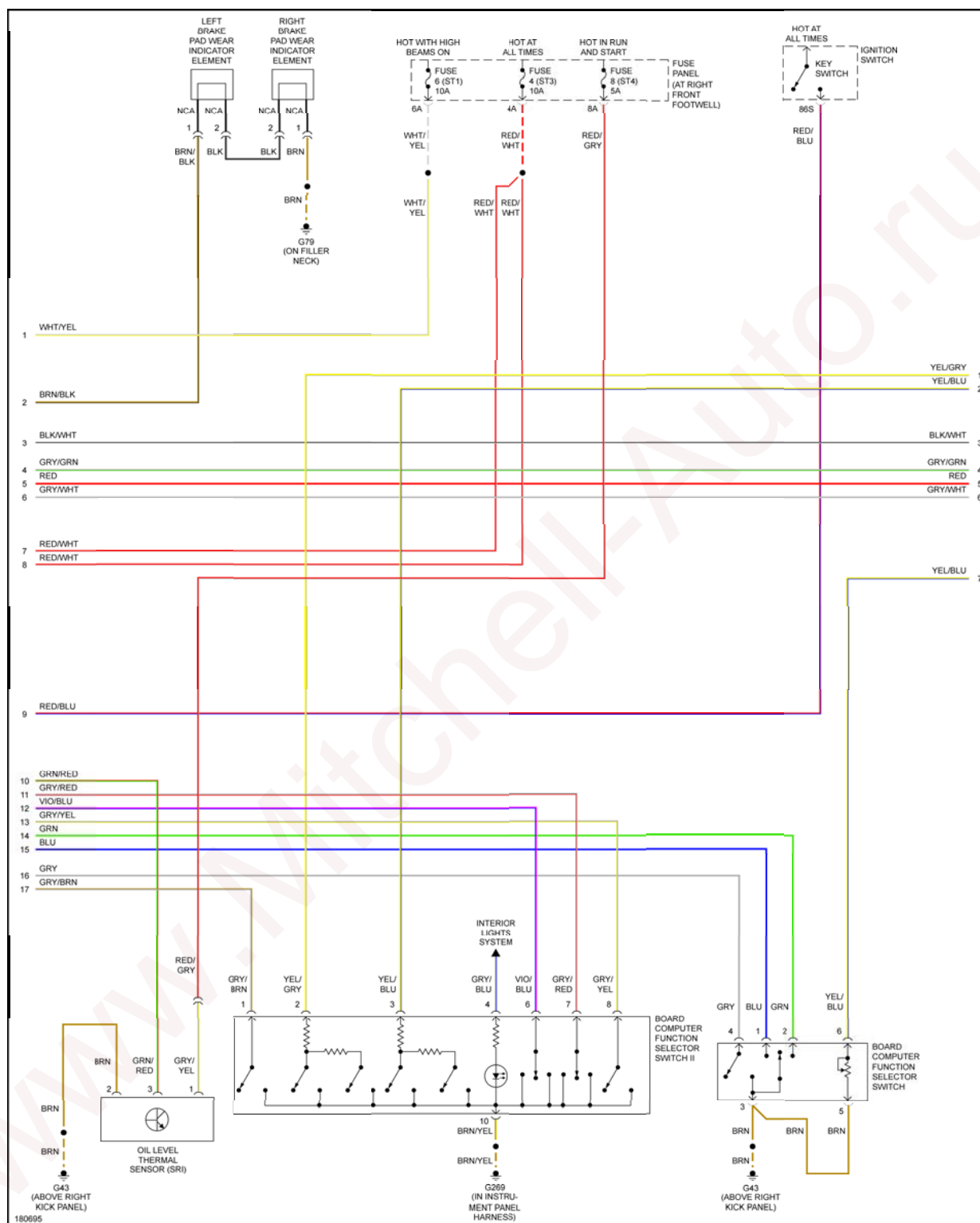
Fig. 28: Instrument Cluster Circuit (2 of 3)
