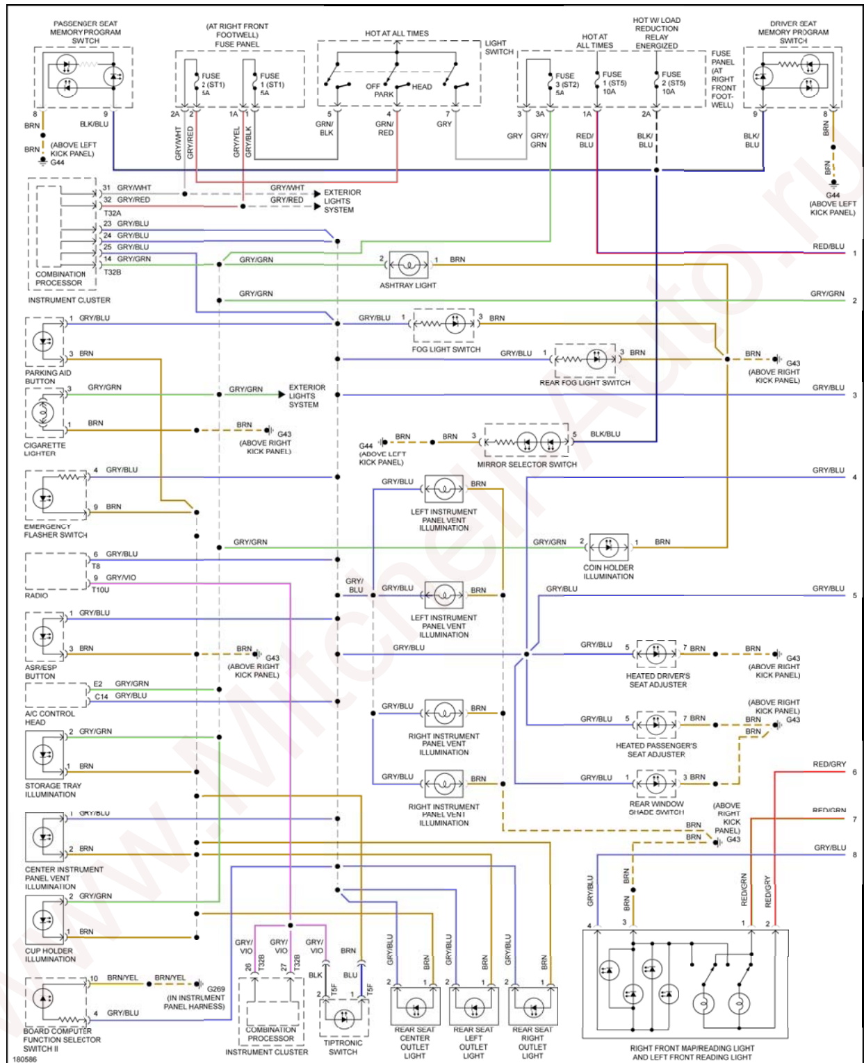
Fig. 30: Interior Lights Circuit (1 of 3)
