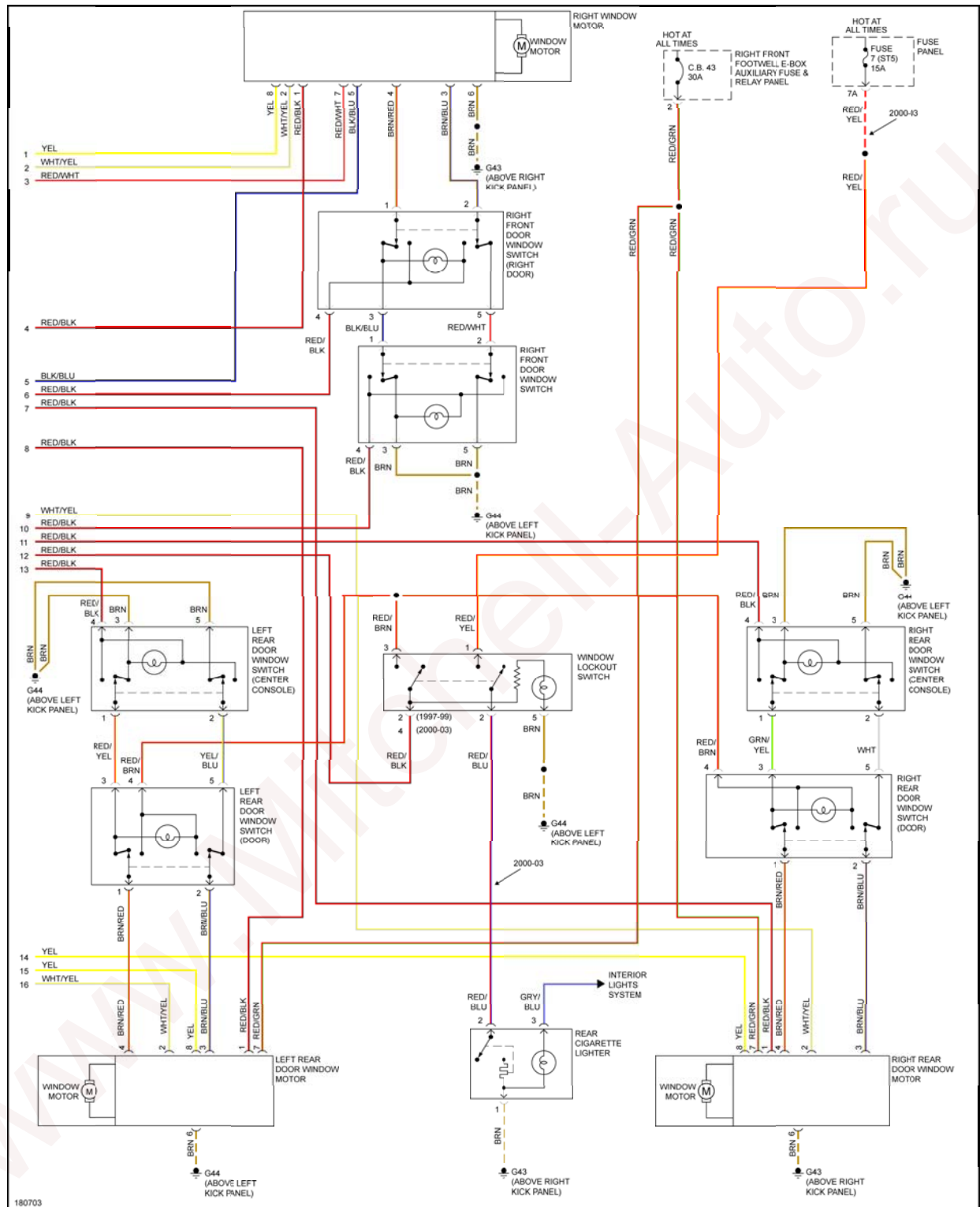
Fig. 55: Power Windows Circuit (2 of 2)
