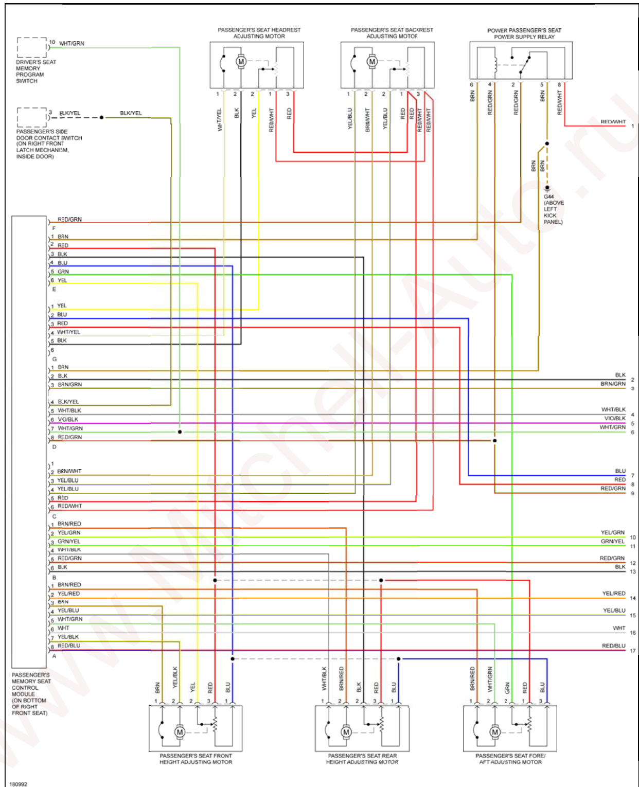
Fig. 37: Passenger's Memory Seat Circuit (1 of 2)
