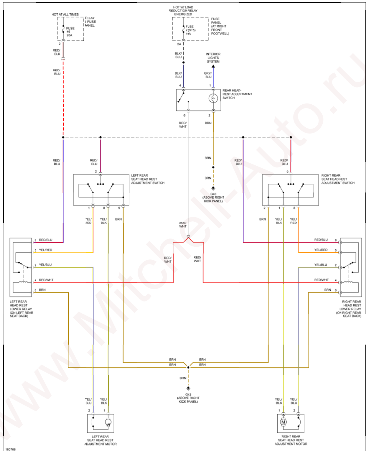
Fig. 52: Rear Power Headrest Circuit
