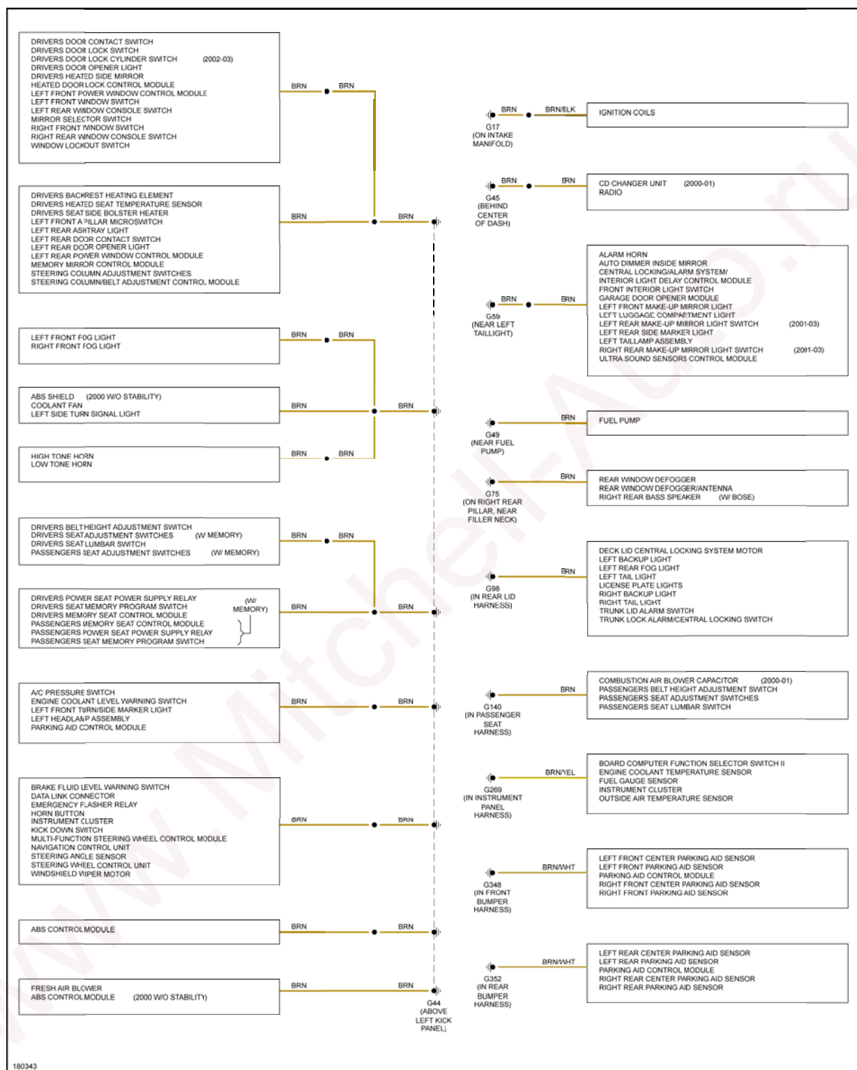
Fig. 22: Ground Distribution Circuit (2 of 2)
