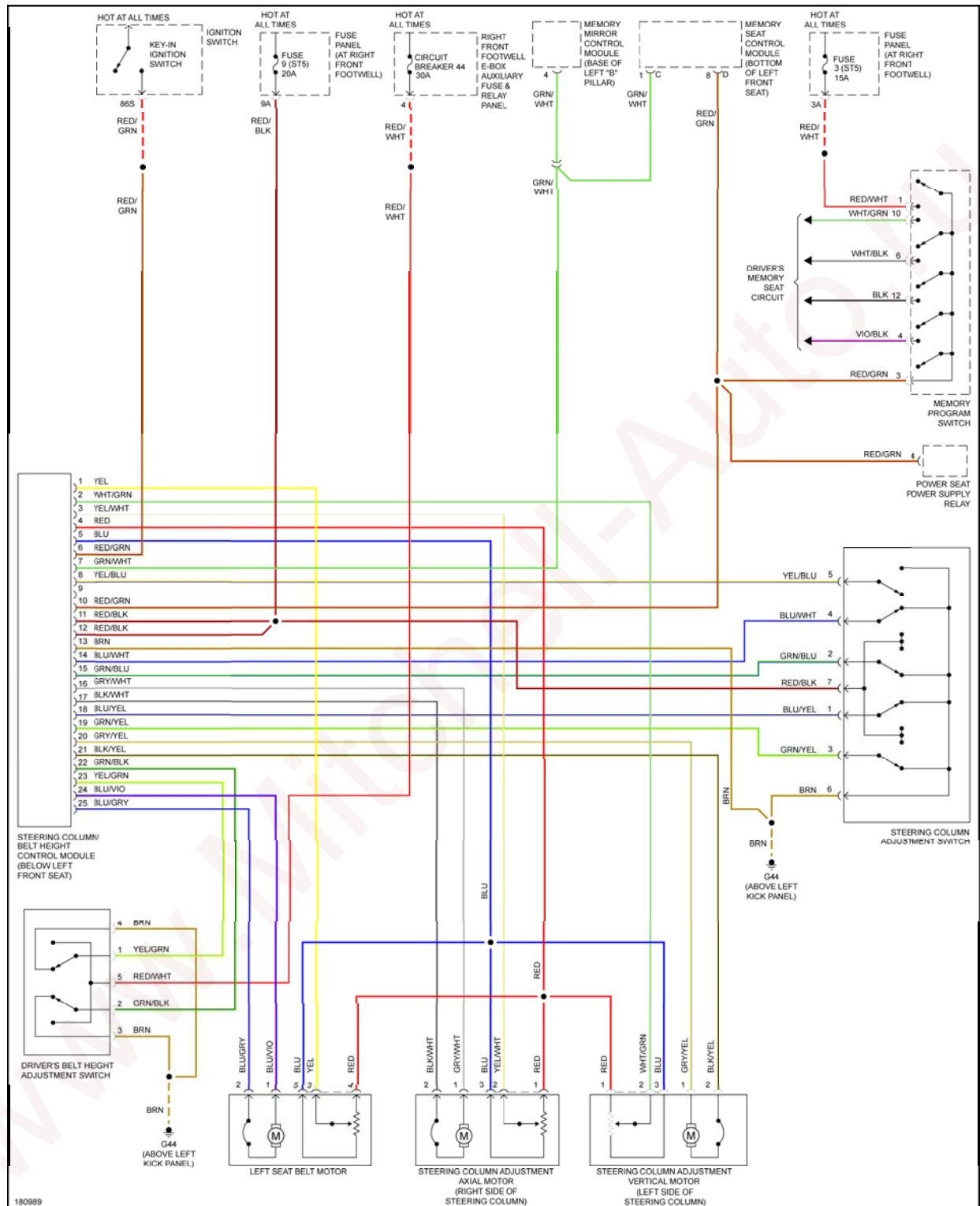
Fig. 35: Memory Column &amp; Belt Height Circuit
