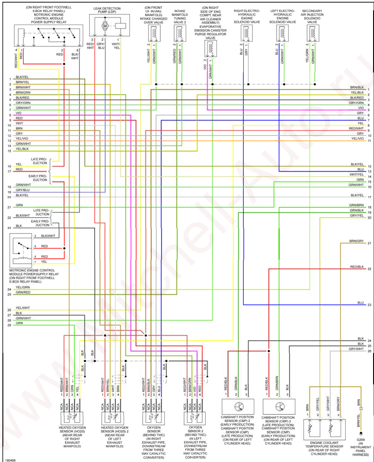
Fig. 13: 4.2L, Engine Performance Circuit (2 of 4)
