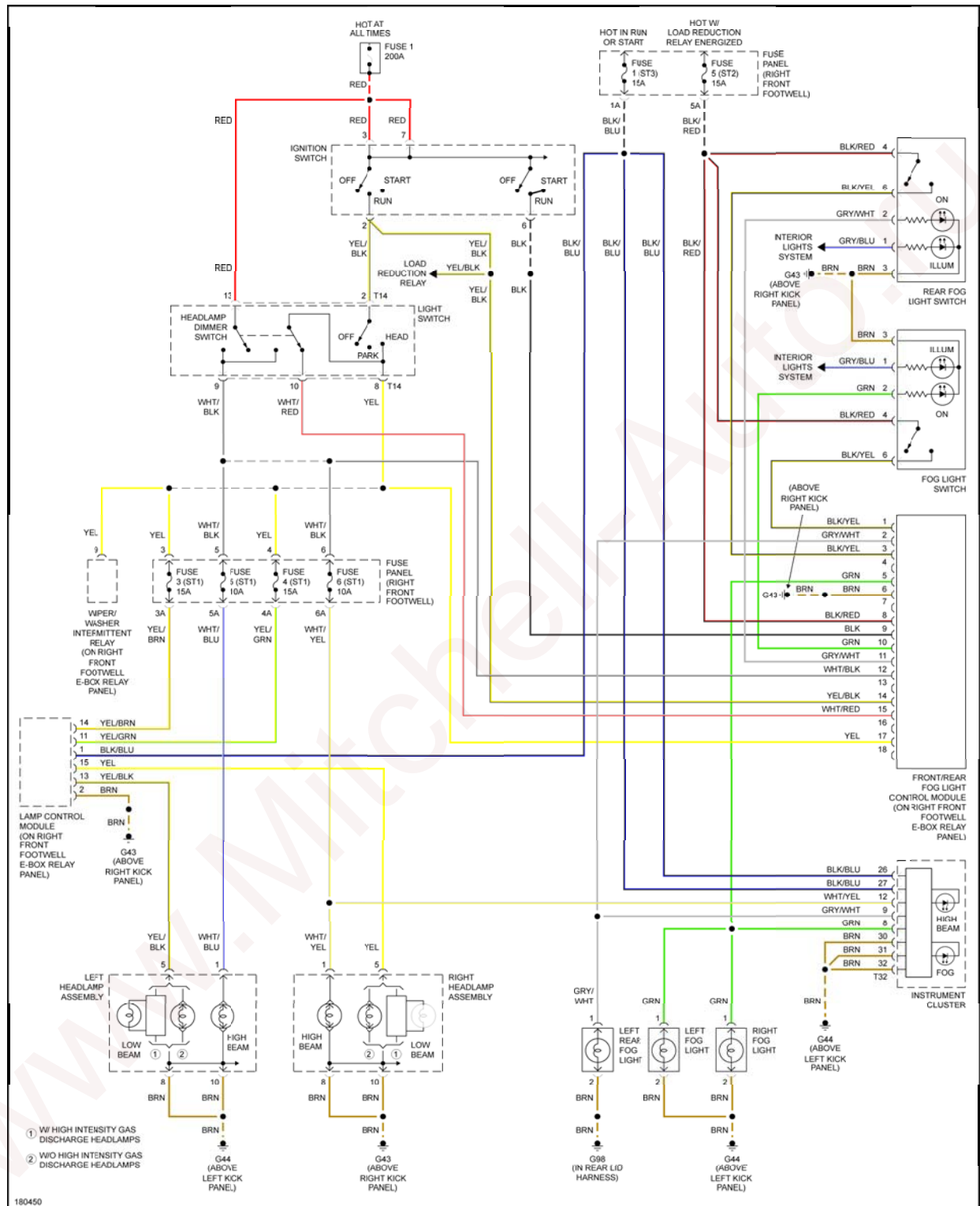
Fig. 25: Headlamps &amp; Fog Lamps Circuit, W/O DRL
