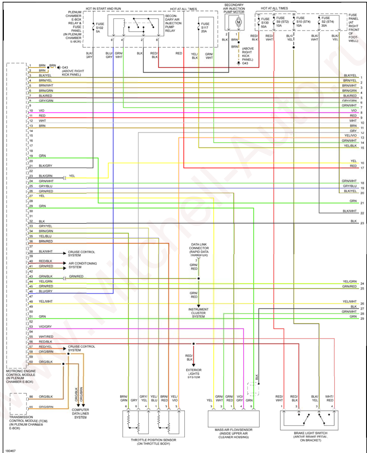
Fig. 12: 4.2L, Engine Performance Circuit (1 of 4)
