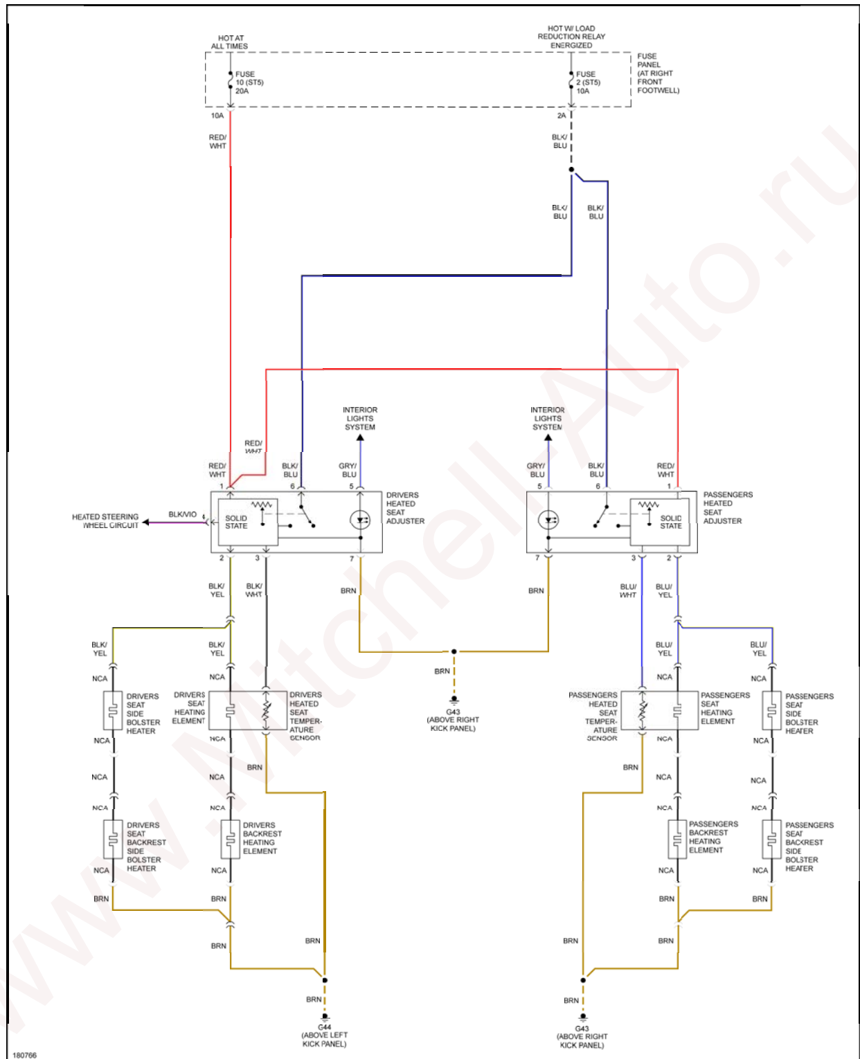
Fig. 47: Front Seat Heater Circuit
