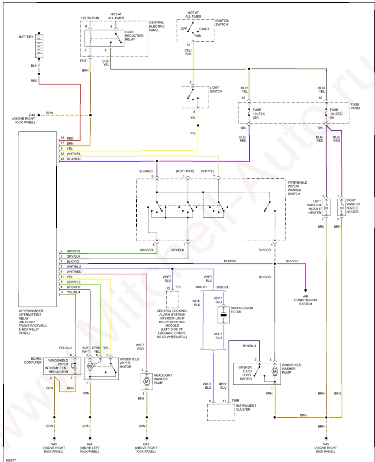
Fig. 66: Wiper/Washer Circuit
