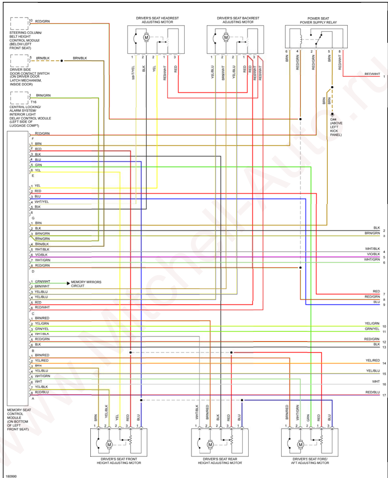
Fig. 33: Driver's Memory Seat Circuit (1 of 2)
