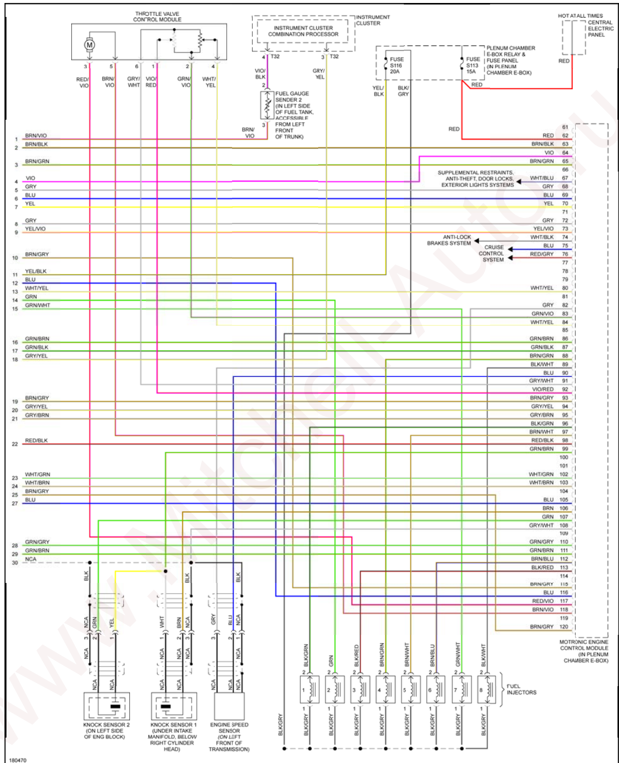
Fig. 15: 4.2L, Engine Performance Circuit (4 of 4)
