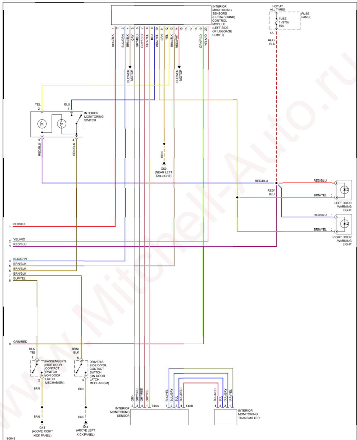
Fig. 5: Power Door Locks Circuit (2 of 2)
