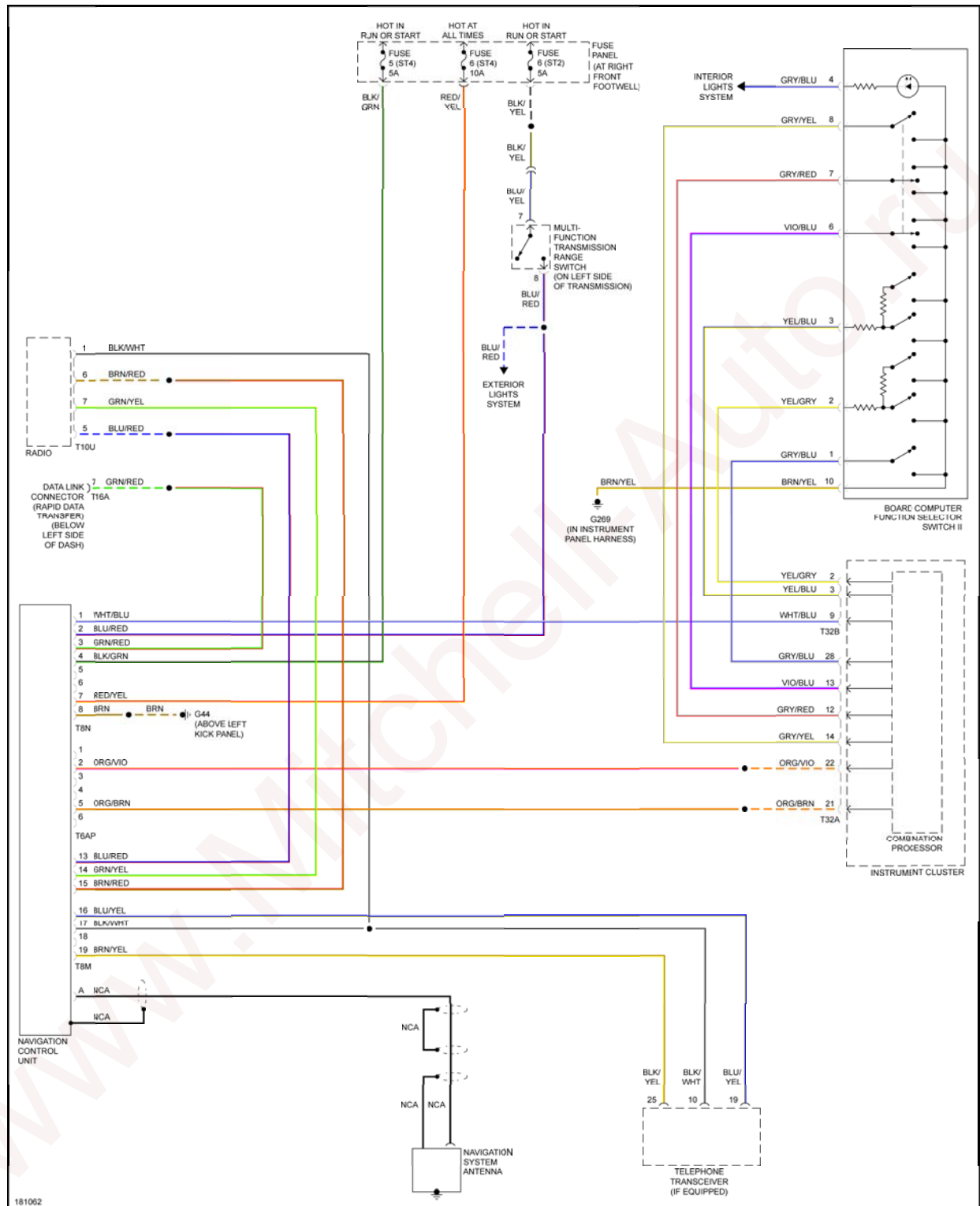
Fig. 39: Navigation Circuit
