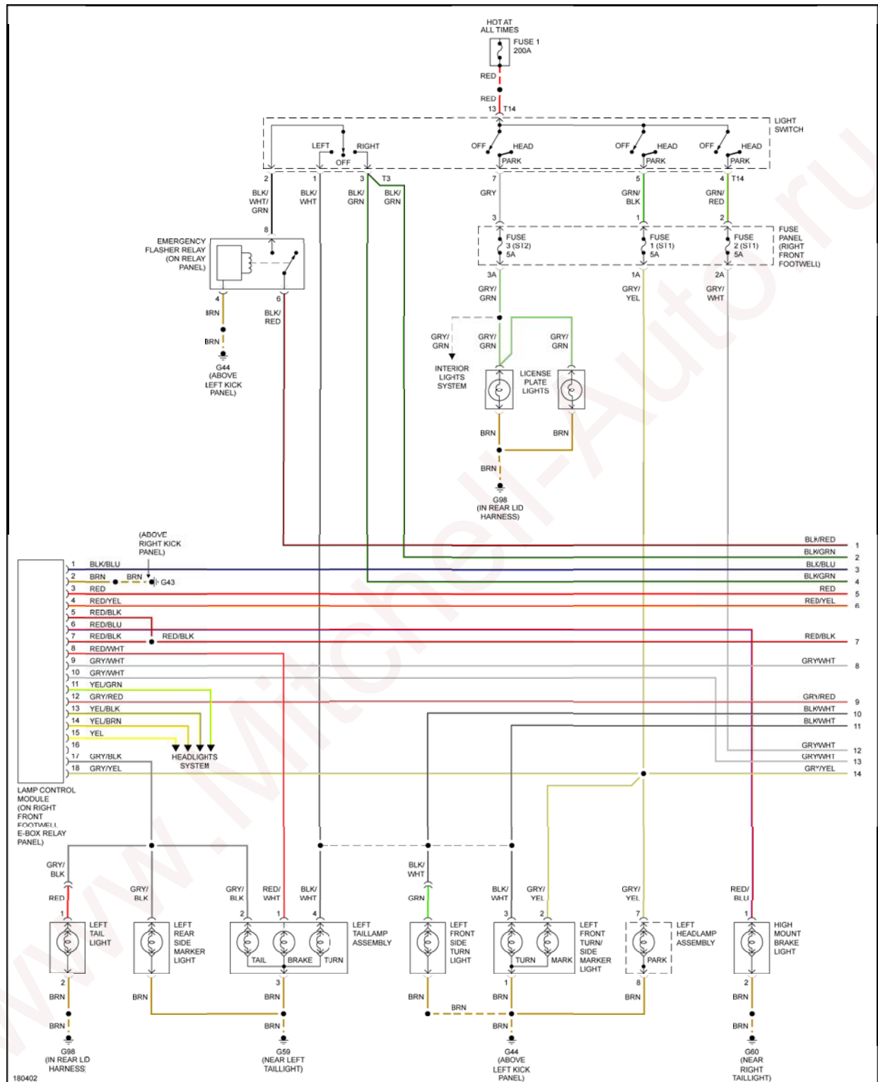
Fig. 19: Exterior Lamps Circuit, W/O DRL (1 of 2)
