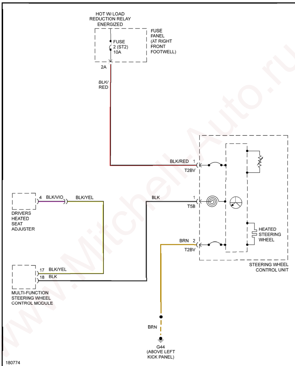
Fig. 48: Heated Steering Wheel Circuit
